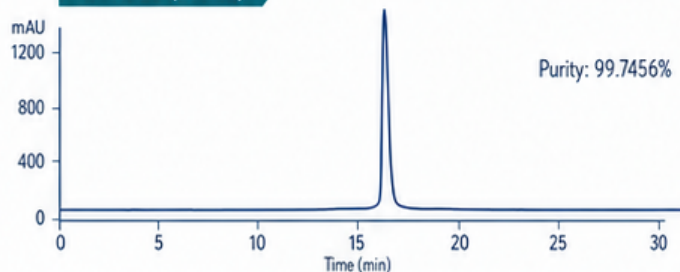
RP-HPLC (214nm)
